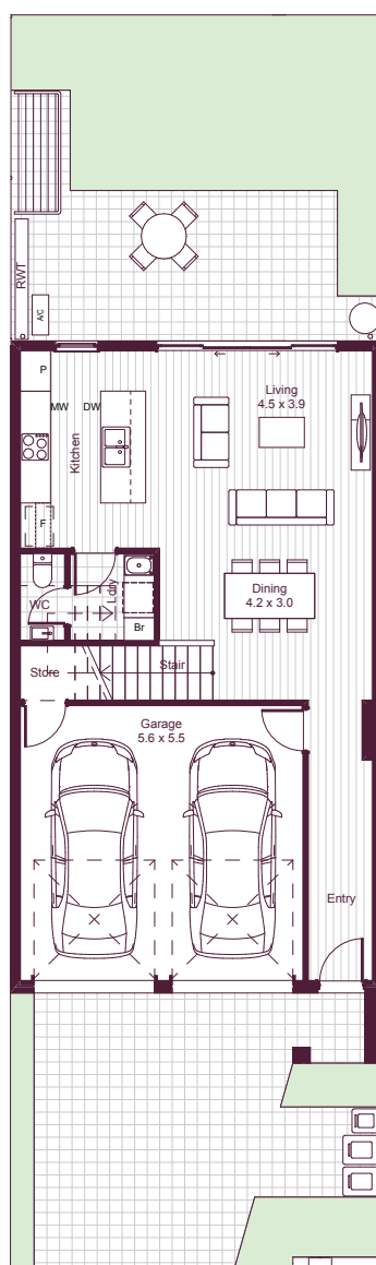
Ground Floor
